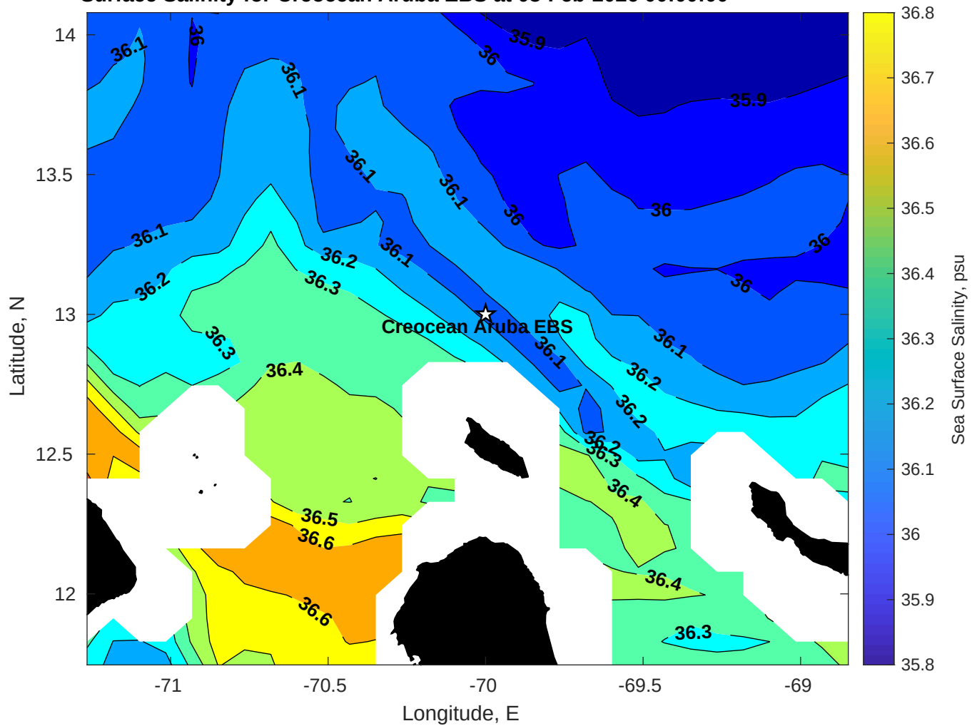
Surface Salinity for Creoccean Aruba EBS at 03-Feb-2026 00:00:00
