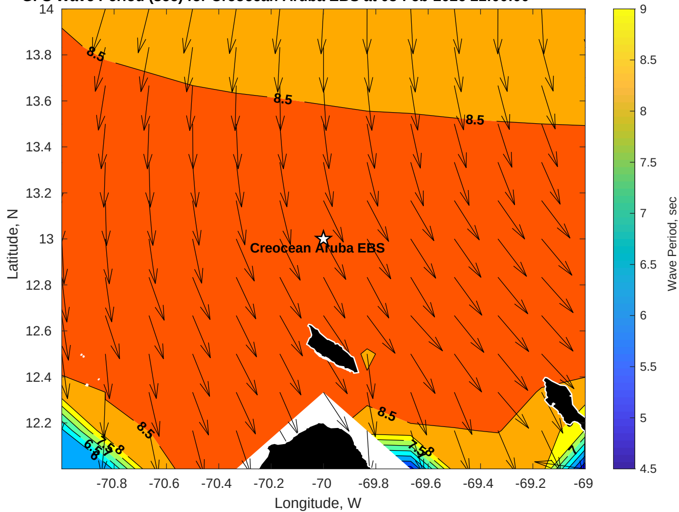
GFS Wave Period (sec) for Creoccean Aruba EBS at 03-Feb-2026 21:00:00
