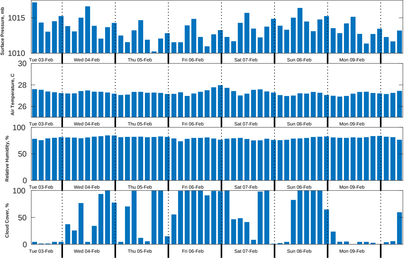
Met Forecast for Creocan Aruba EBS from 03-Feb-2026 12:00:00 to 10-Feb-2026 12:00:00
