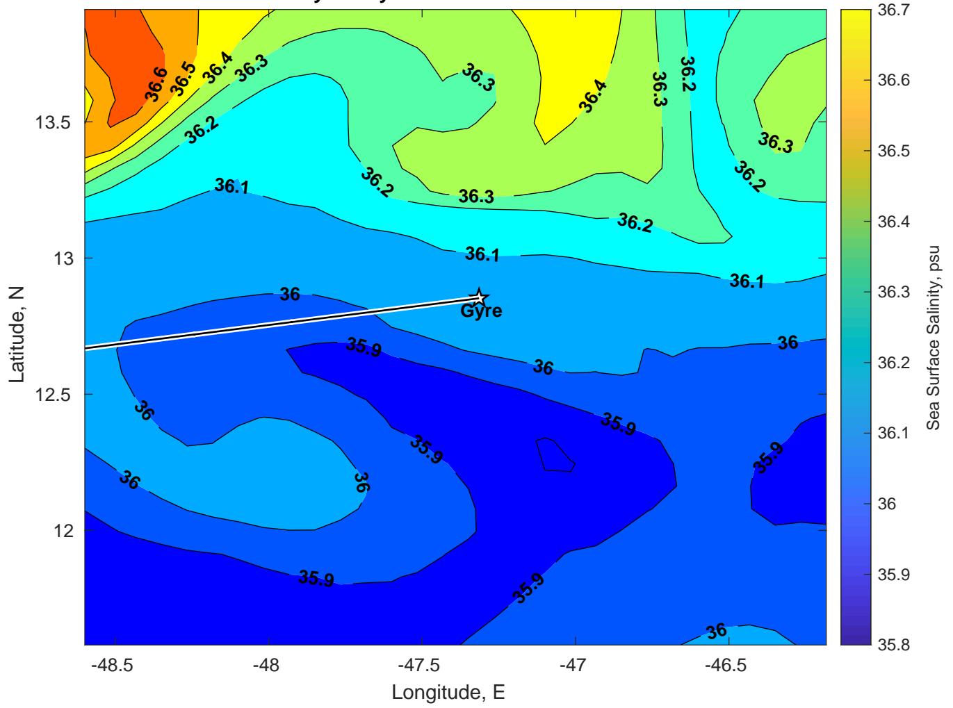
Surface Salinity for Gyre at 17-Jan-2025 00:00:00
