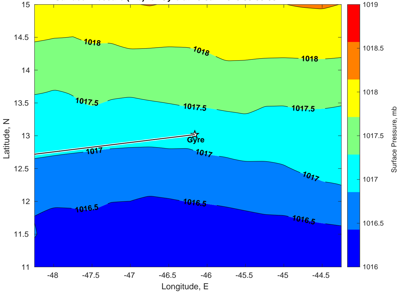
Surface Pressure (mb) for Gyre at 19-Jan-2025 00:00:00
