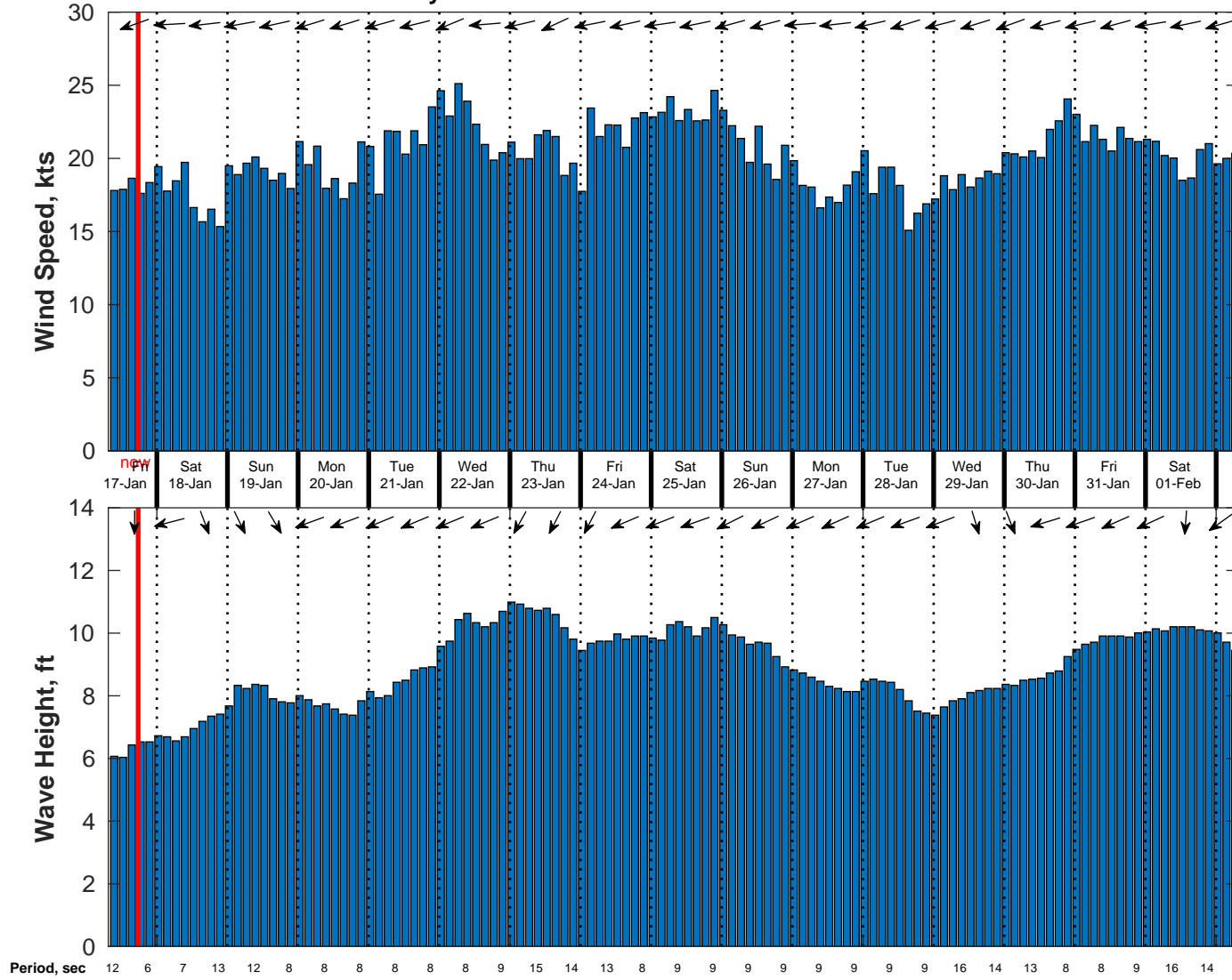
Wind & Wave Forecast for Gyre from 17-Jan-2025 08:00:00 to 02-Feb-2025 08:00:00
