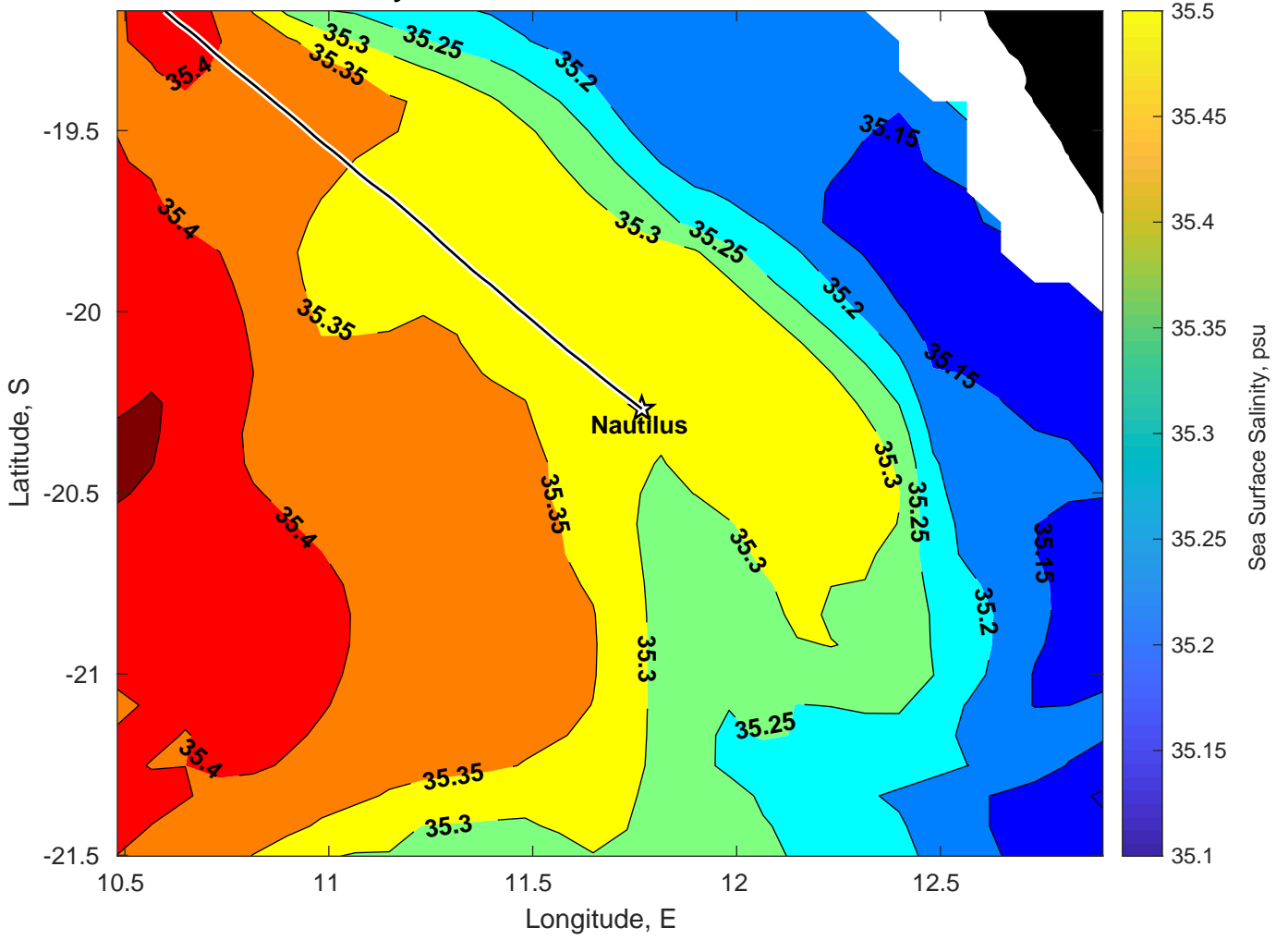
Surface Salinity for Nautilus at 17-Jan-2025 00:00:00
