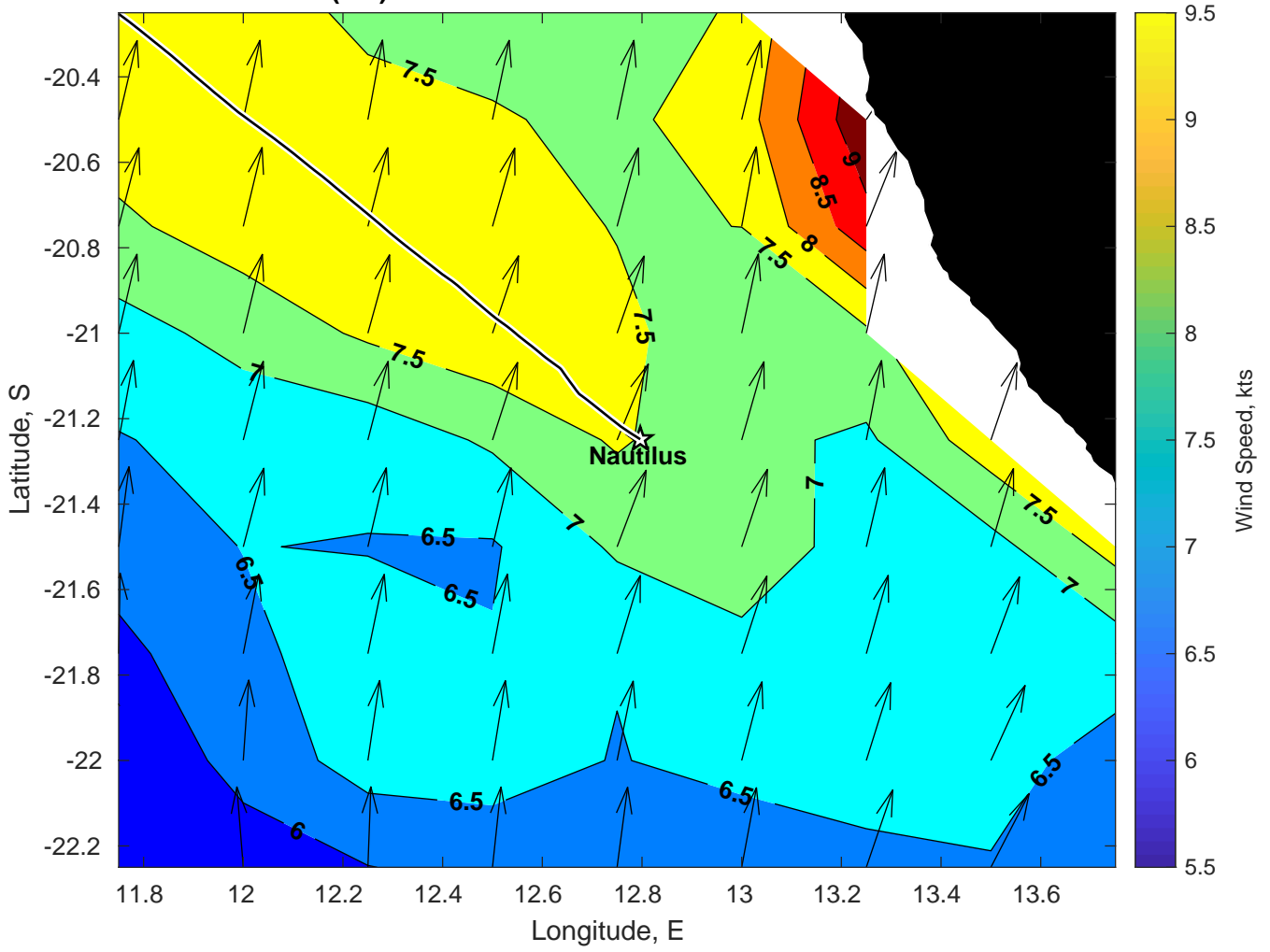
Winds (kts) for Nautilus at 18-Jan-2025 09:00:00
