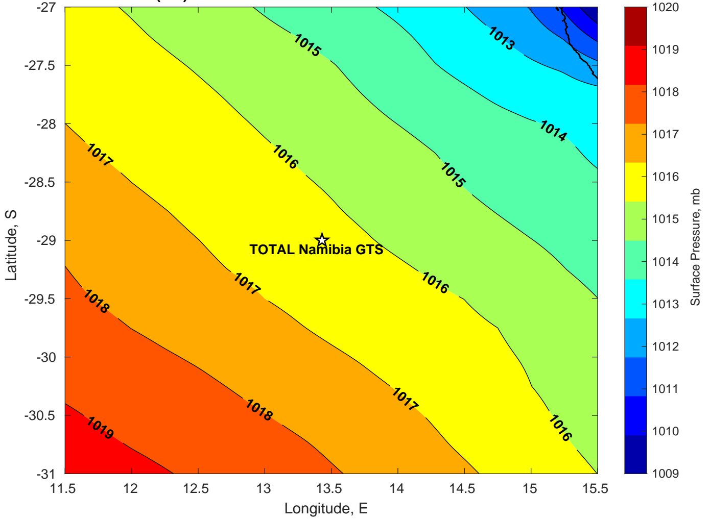
Surface Pressure (mb) for TOTAL Namibia GTS at 24-Feb-2025 12:00:00
