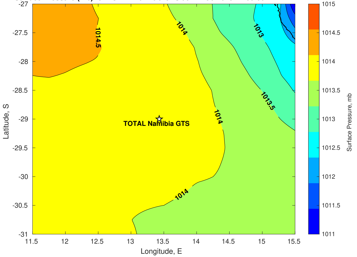
Surface Pressure (mb) for TOTAL Namibia GTS at 22-Feb-2025 12:00:00
