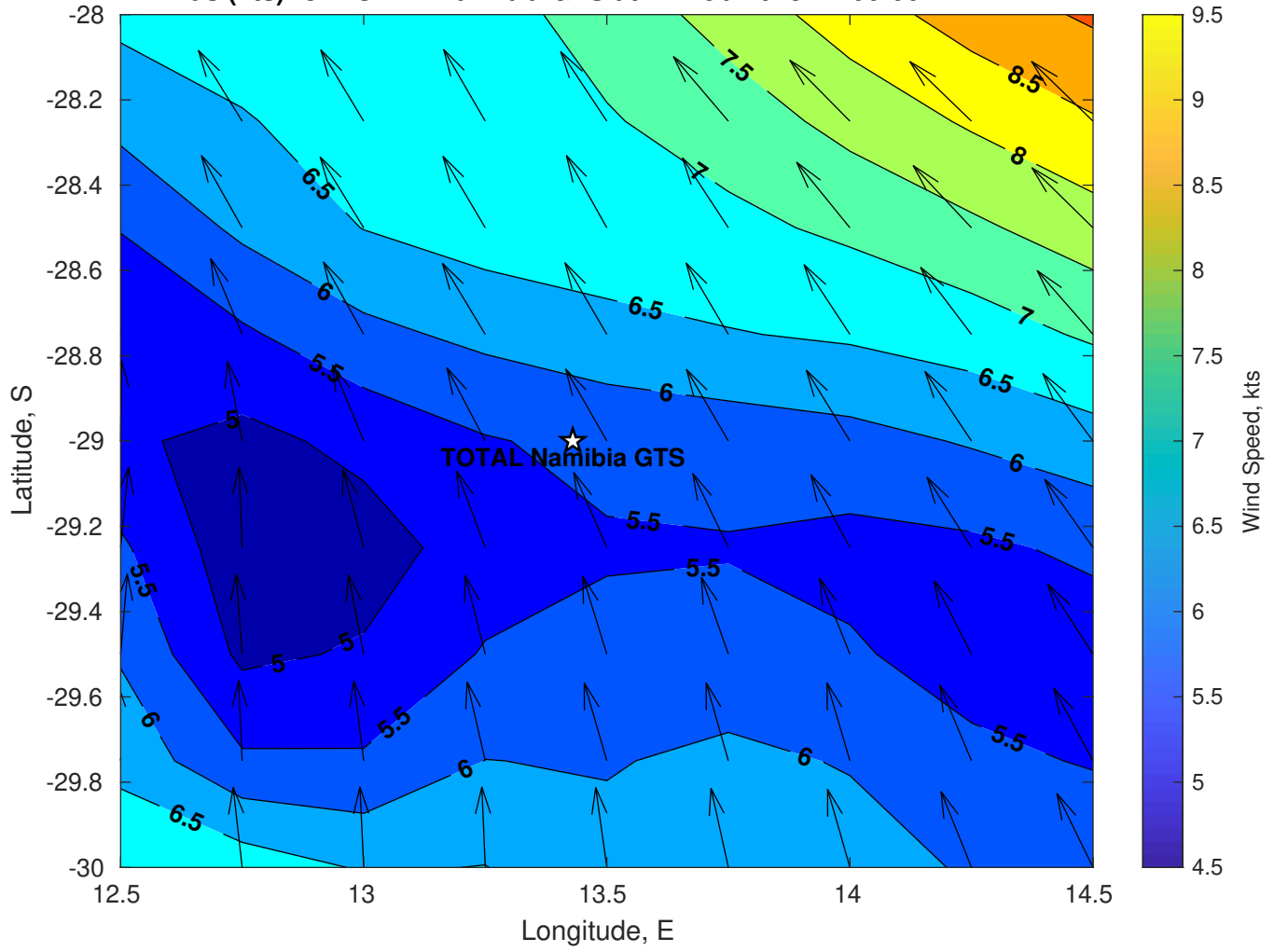
Winds (kts) for TOTAL Namibia GTS at 22-Feb-2025 21:00:00
