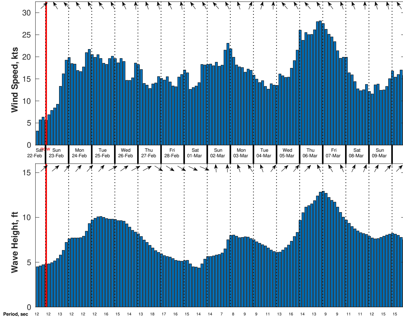
Wind & Wave Forecast for TOTAL Namibia GTS from 22-Feb-2025 14:00:00 to 10-Mar-2025 14:00:00
