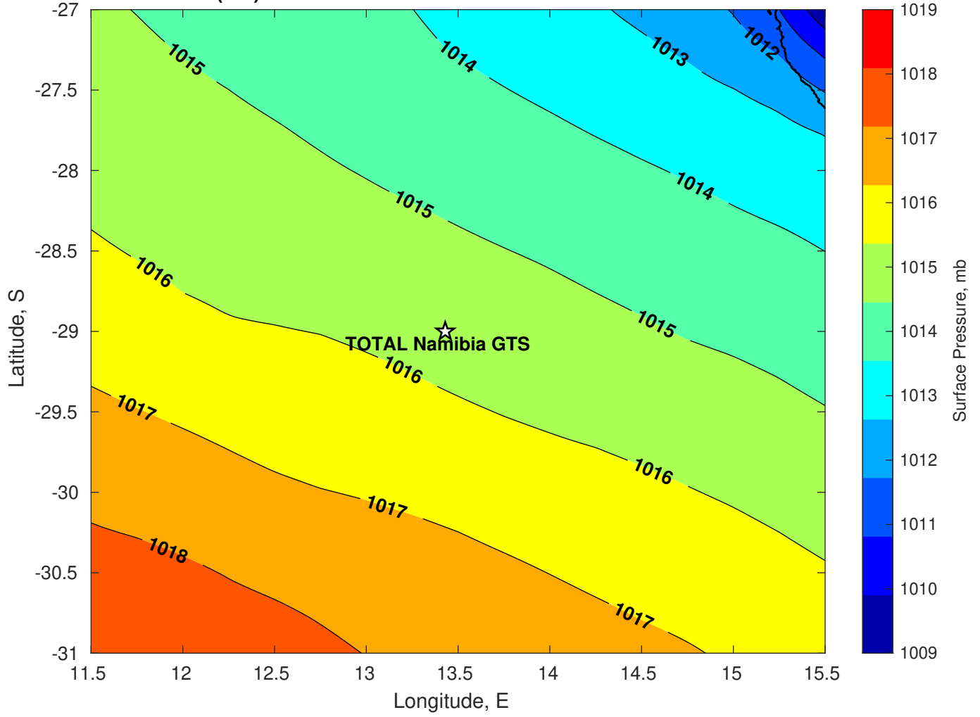
Surface Pressure (mb) for TOTAL Namibia GTS at 23-Feb-2025 12:00:00
