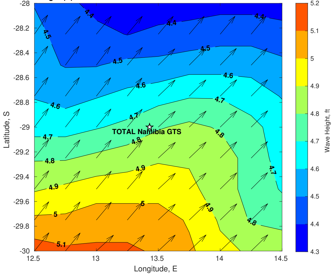
Wave Height (ft) for TOTAL Namibia GTS at 22-Feb-2025 21:00:00
