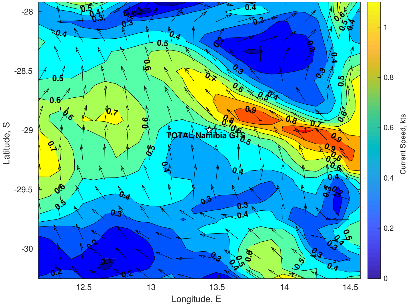
Surface Currents for TOTAL Namibia GTS at 22-Feb-2025 00:00:00
