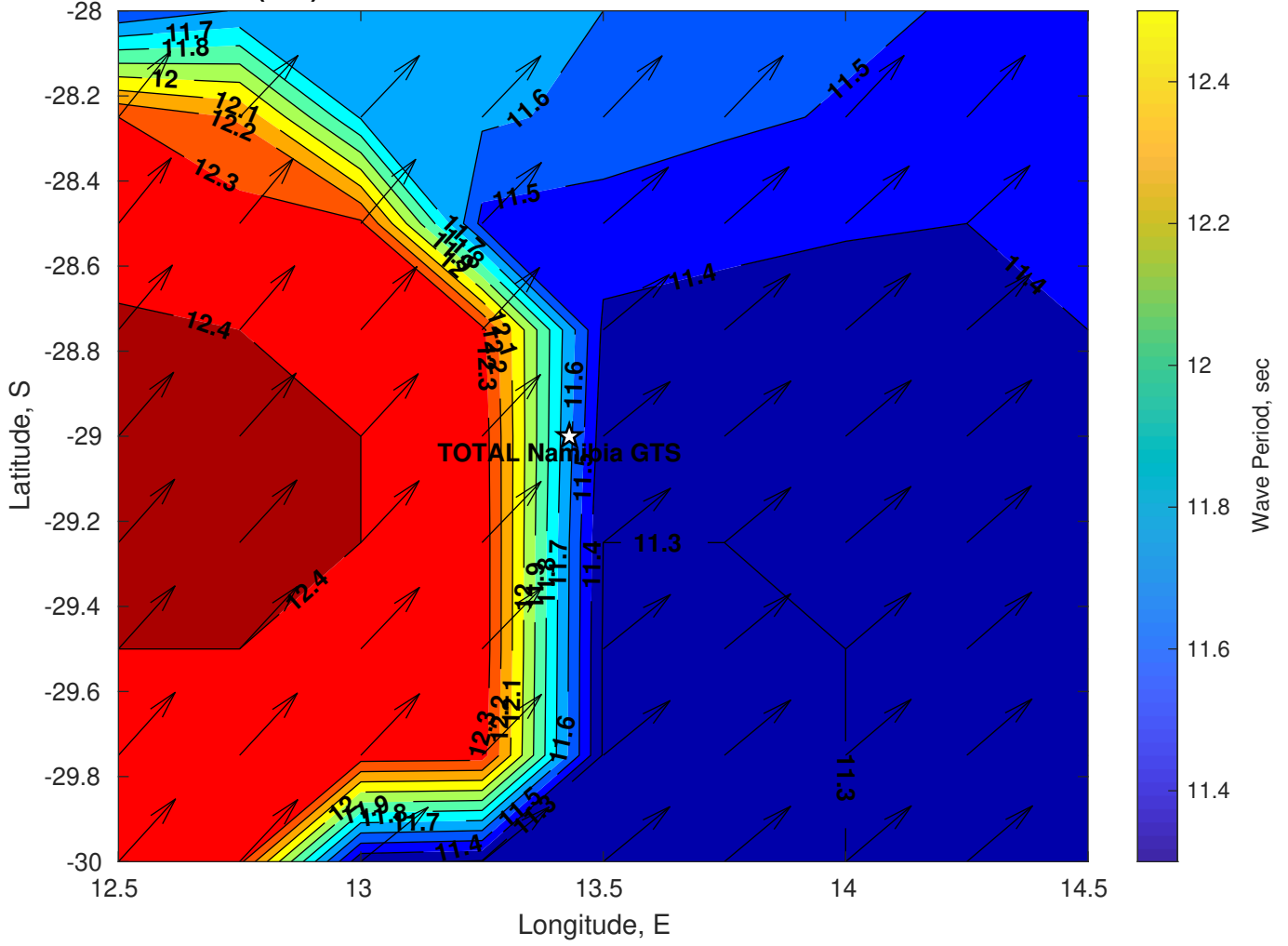
Wave Period (sec) for TOTAL Namibia GTS at 22-Feb-2025 21:00:00
