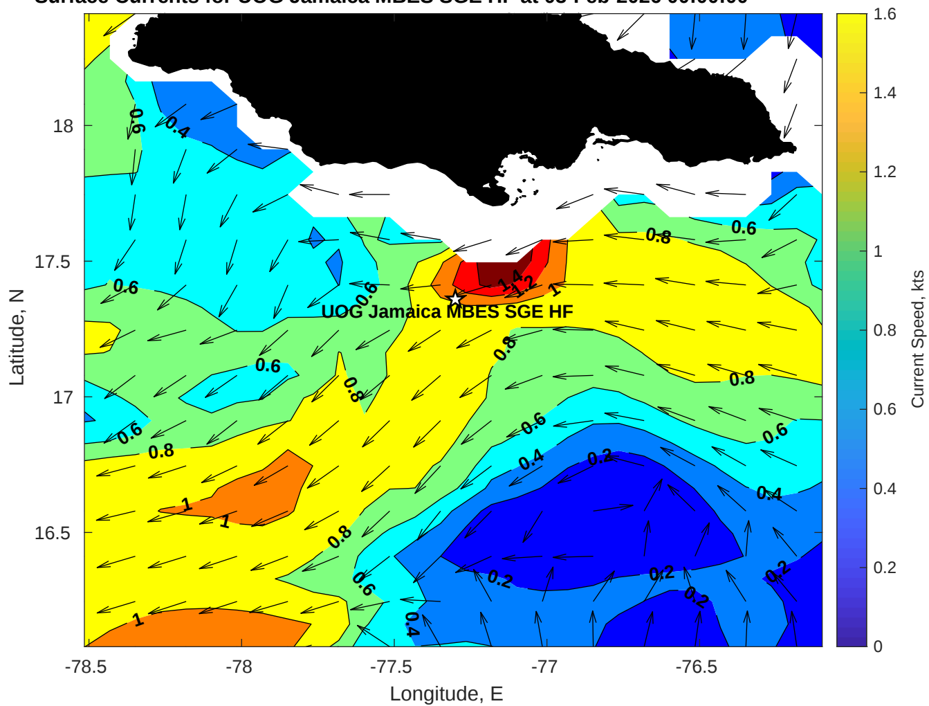
Surface Currents for UOG Jamaica MBES SGE HF at 03-Feb-2026 00:00:00
