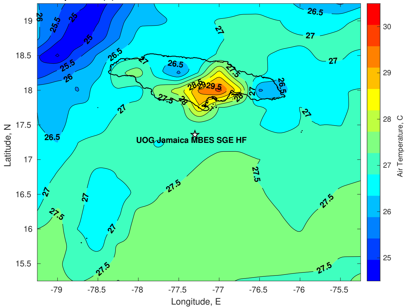
Air Temperature (C) for UOG Jamaica MBES SGE HF at 03-Feb-2026
