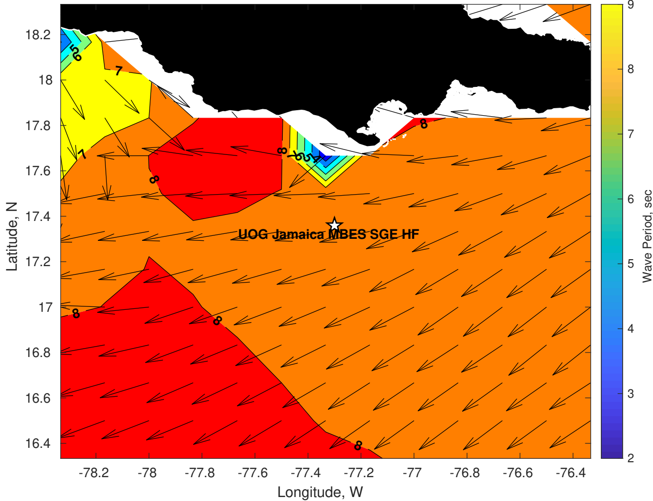
GFS Wave Period (sec) for UOG Jamaica MBES SGE HF at 03-Feb-2026 21:00:00
