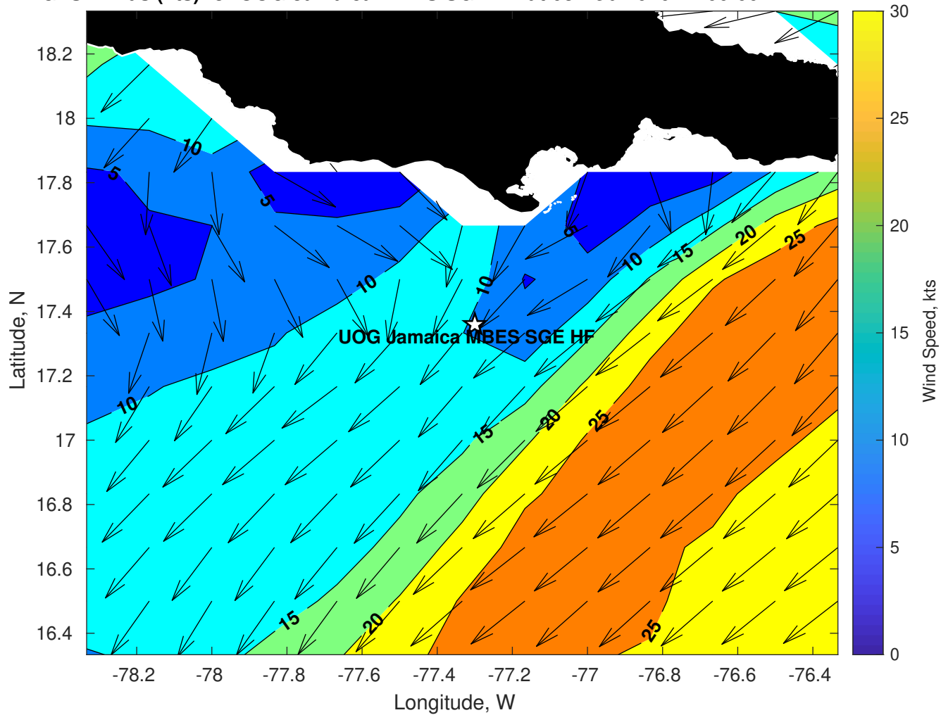
GFS Winds (kts) for UOG Jamaica MBES SGE HF at 03-Feb-2026 21:00:00
