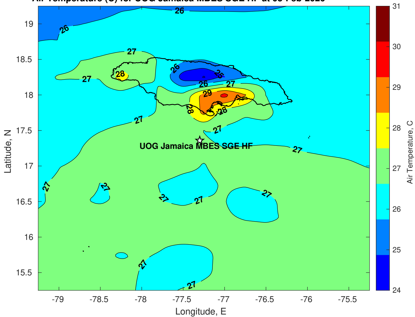
Air Temperature (C) for UOG Jamaica MBES SGE HF at 03-Feb-2026
