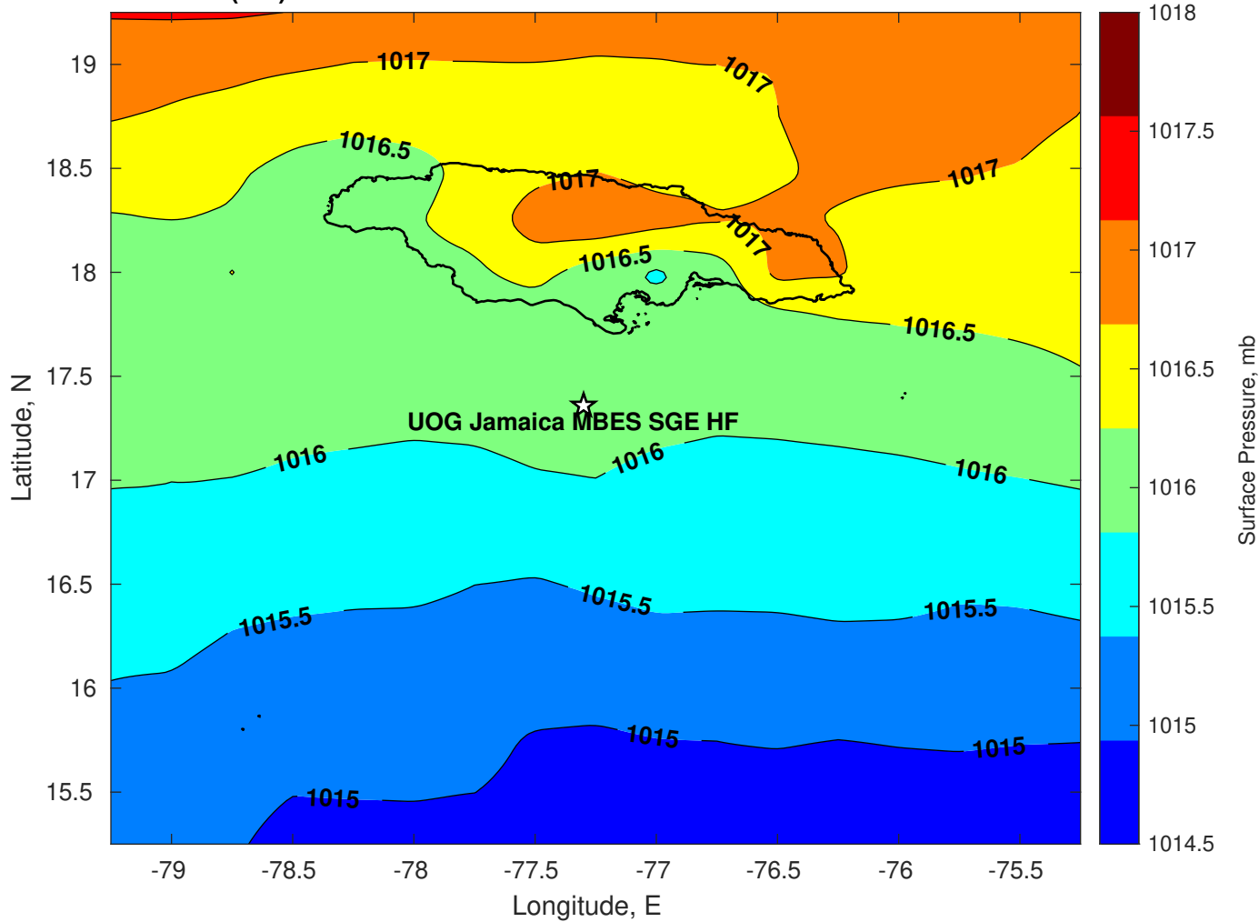
Surface Pressure (mb) for UOG Jamaica MBES SGE HF at 04-Feb-2026 18:00:00
