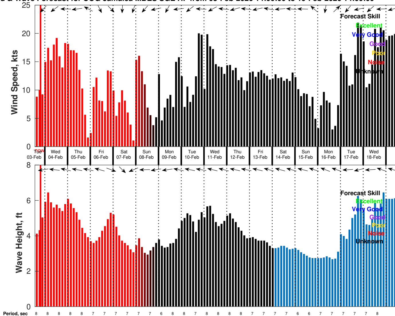
Wind & Wave Forecast for UOG Jamaica MBES SGE HF from 03-Feb-2026 14:00:00 to 19-Feb-2026 14:00:00
