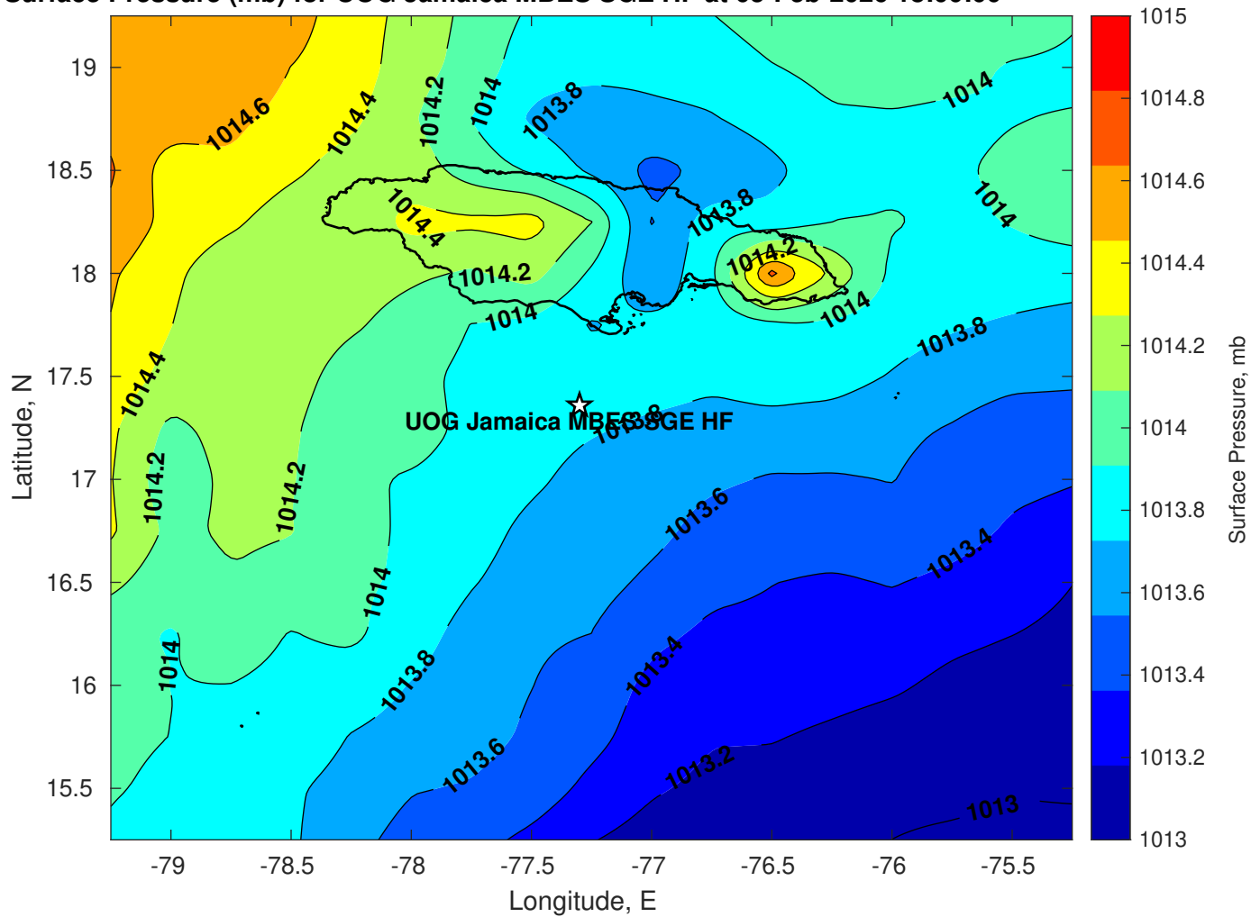
Surface Pressure (mb) for UOG Jamaica MBES SGE HF at 05-Feb-2026 18:00:00
