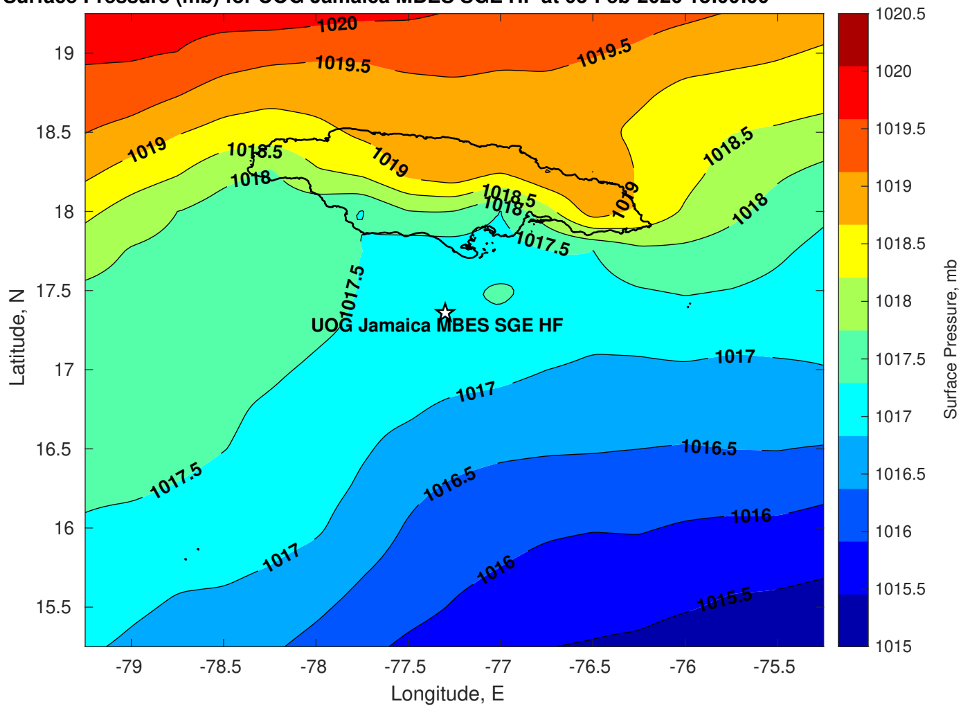
Surface Pressure (mb) for UOG Jamaica MBES SGE HF at 03-Feb-2026 18:00:00
