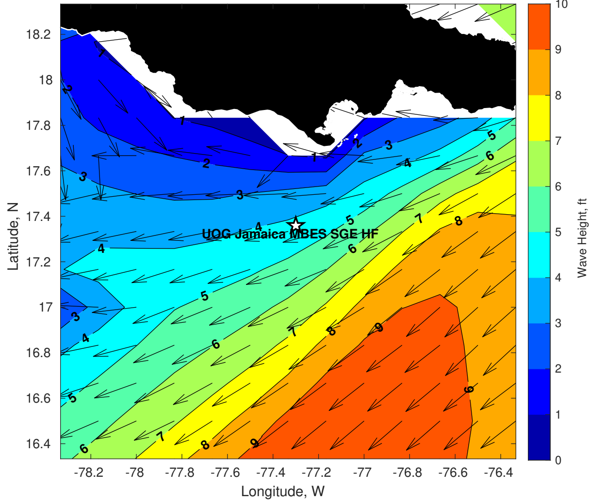
GFS Wave Height (ft) for UOG Jamaica MBES SGE HF at 03-Feb-2026 21:00:00
