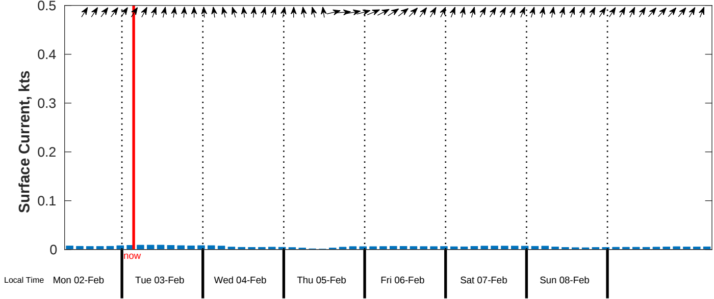
Surface Current Forecast for UOG Jamaica MBES SGE HF from 03-Feb-2026 00:00:00 to 11-Feb-2026 00:00:00
